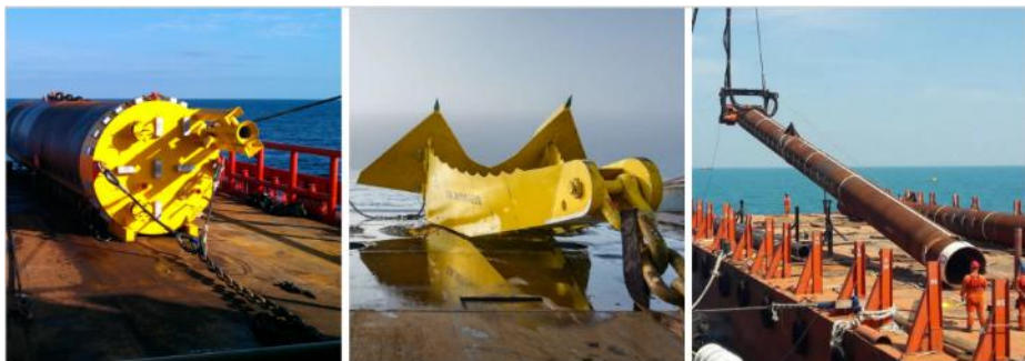
Figure 29 Suction pile anchor, drag embedment anchor and driven pile anchor. Images courtesy of Acteon, Principle Power and Acteon. All rights reserved.
